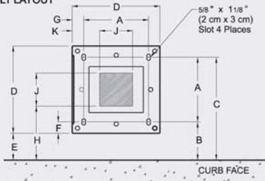
BOLT LAYOUT
