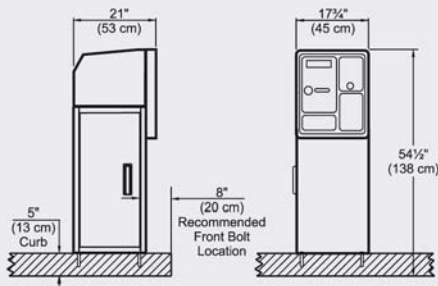
BOLT LAYOUT
